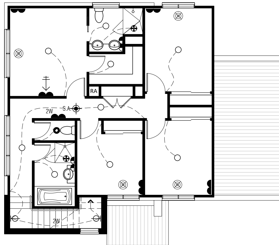
UPPER FLOOR PLAN - OPTION 1 (4 BEDROOM - 1 LIVING)
