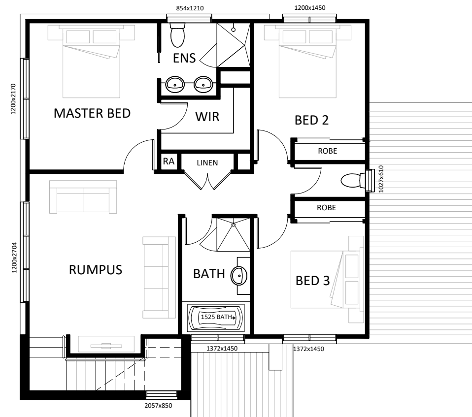
UPPER FLOOR PLAN - OPTION 2 (3 BEDROOM - 2 LIVING)
